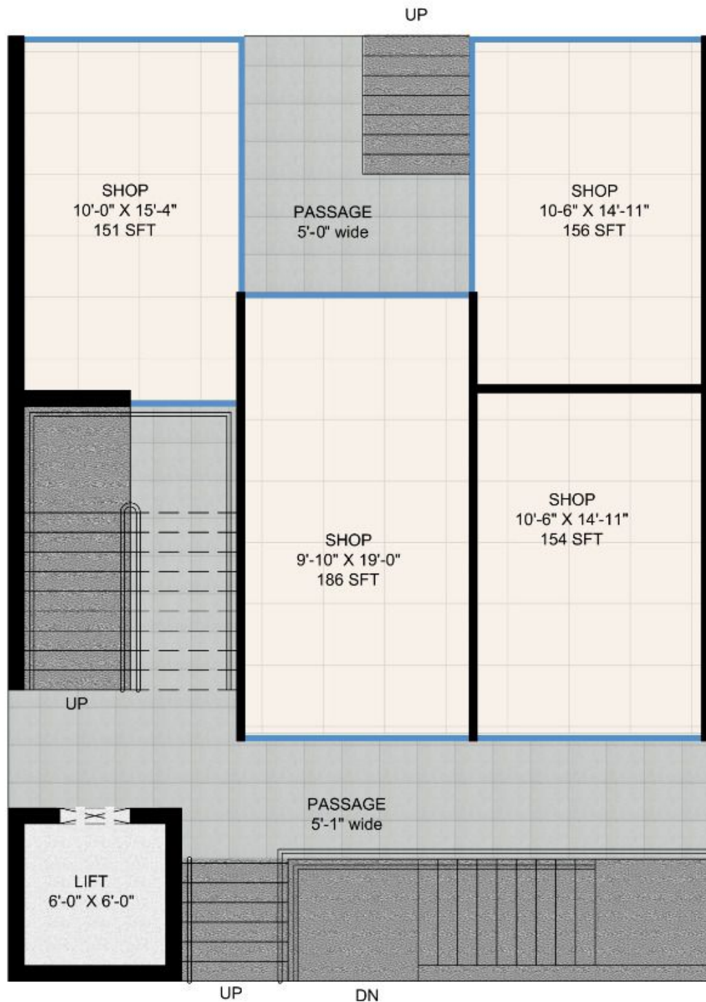
GROUND FLOOR PLAN (HALL)
